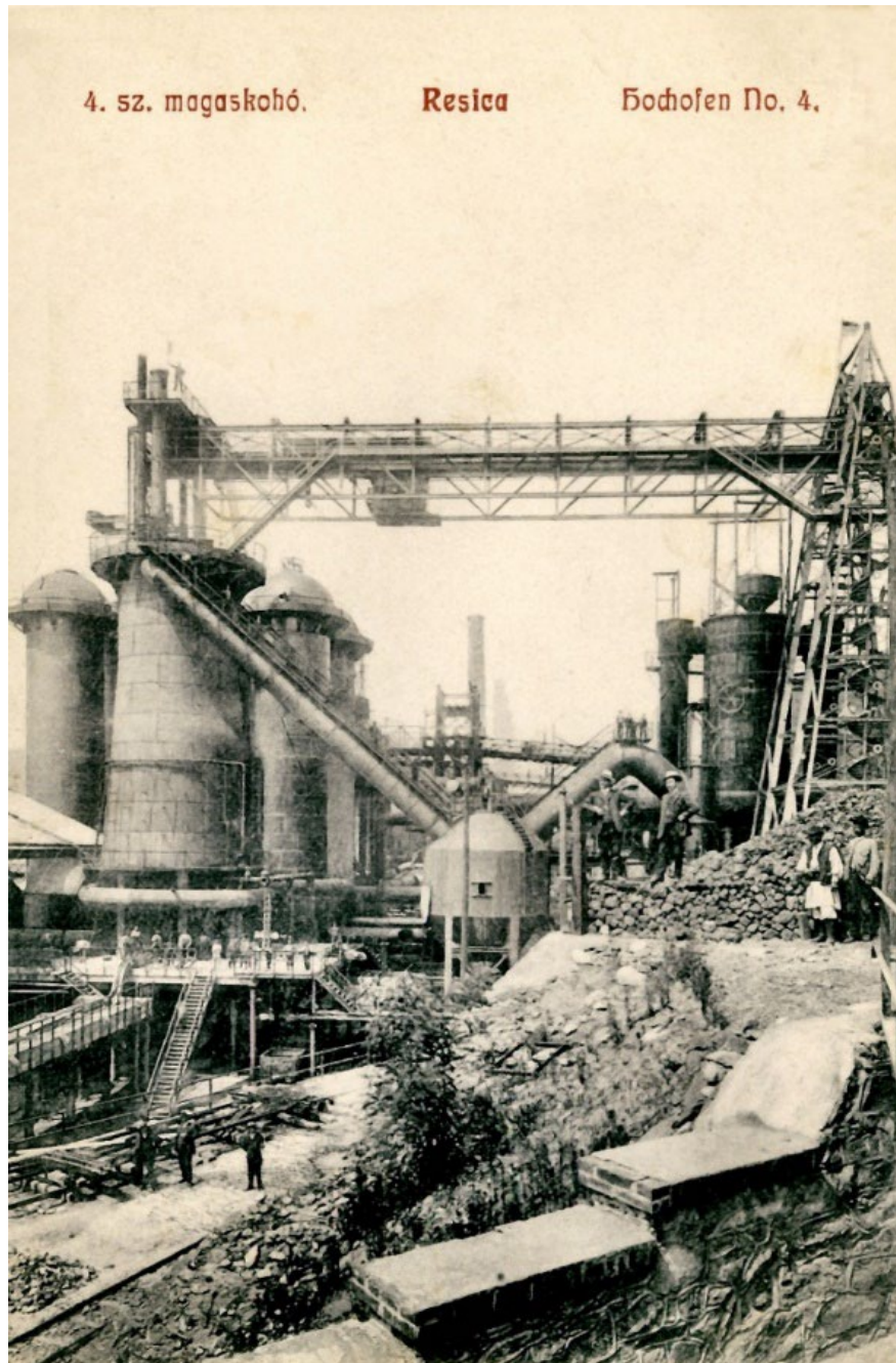
Figure 6 Smelter No. 4, 1912; Kulhanek collection
